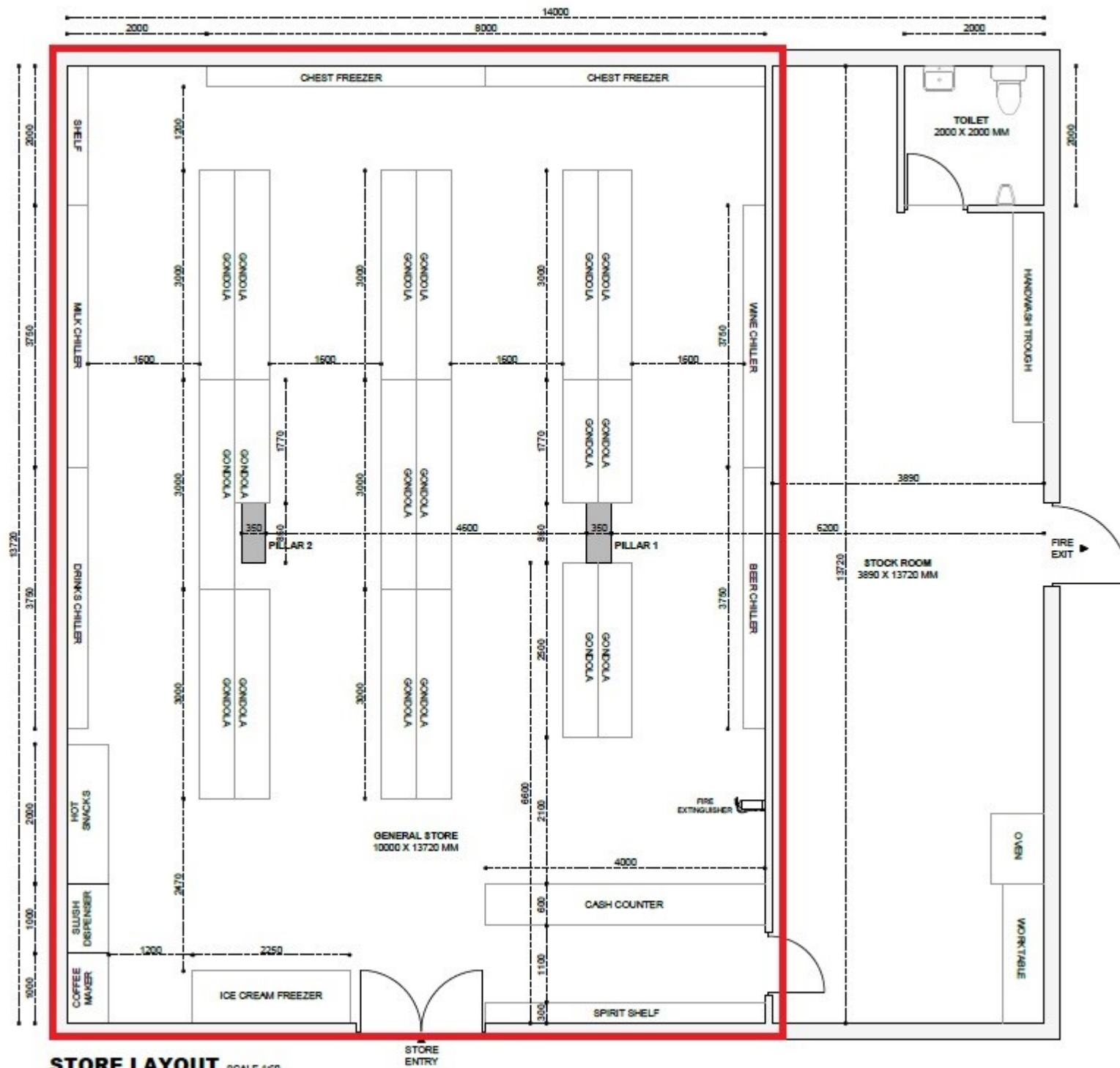
STORE LAYOUT SCALE 1:50
